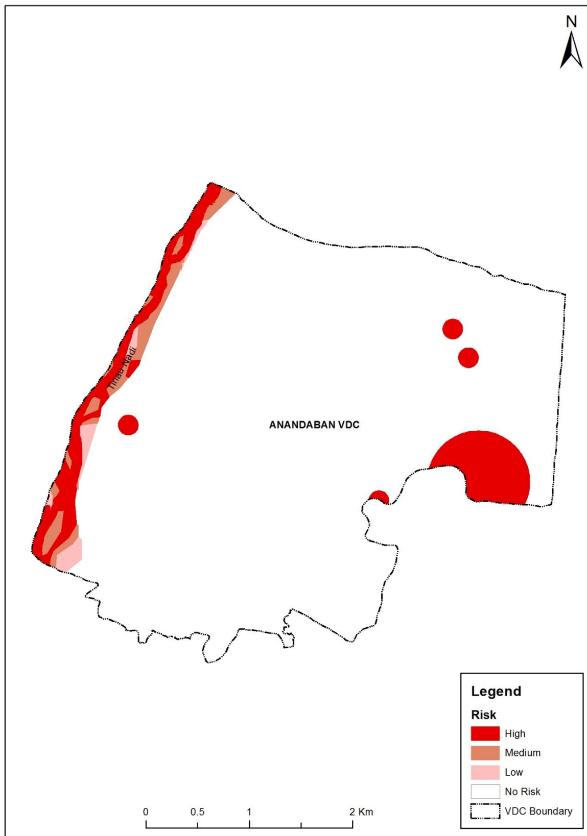
Figure 4.1 Composite of risk layers in Anandaban VDC
