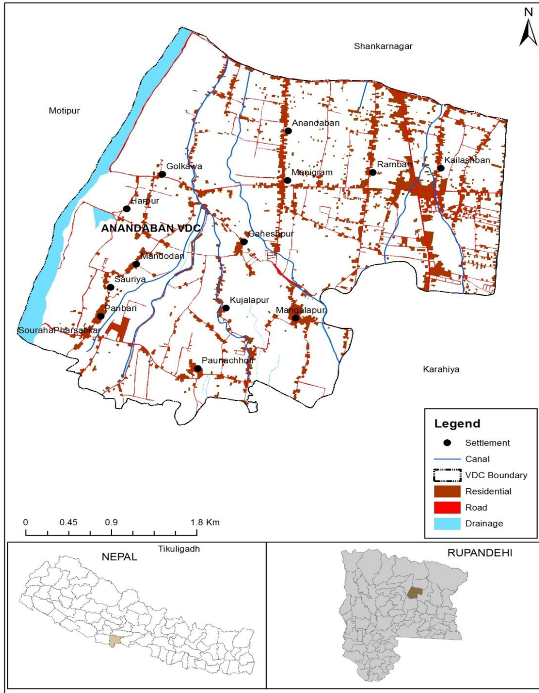
Figure 1.1 Location of Anandaban VDC
