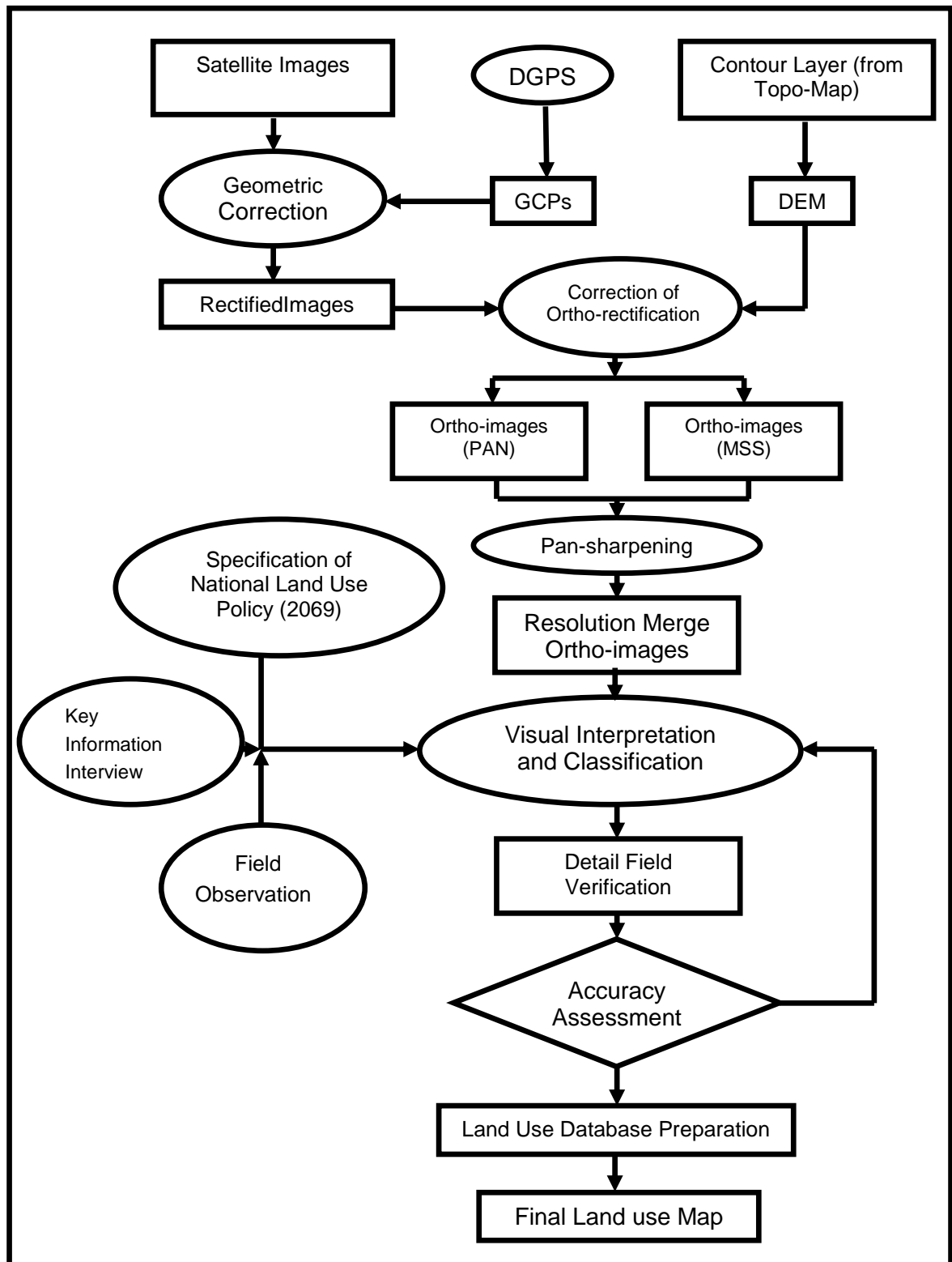
Figure 3.4 Work Flow Diagram
