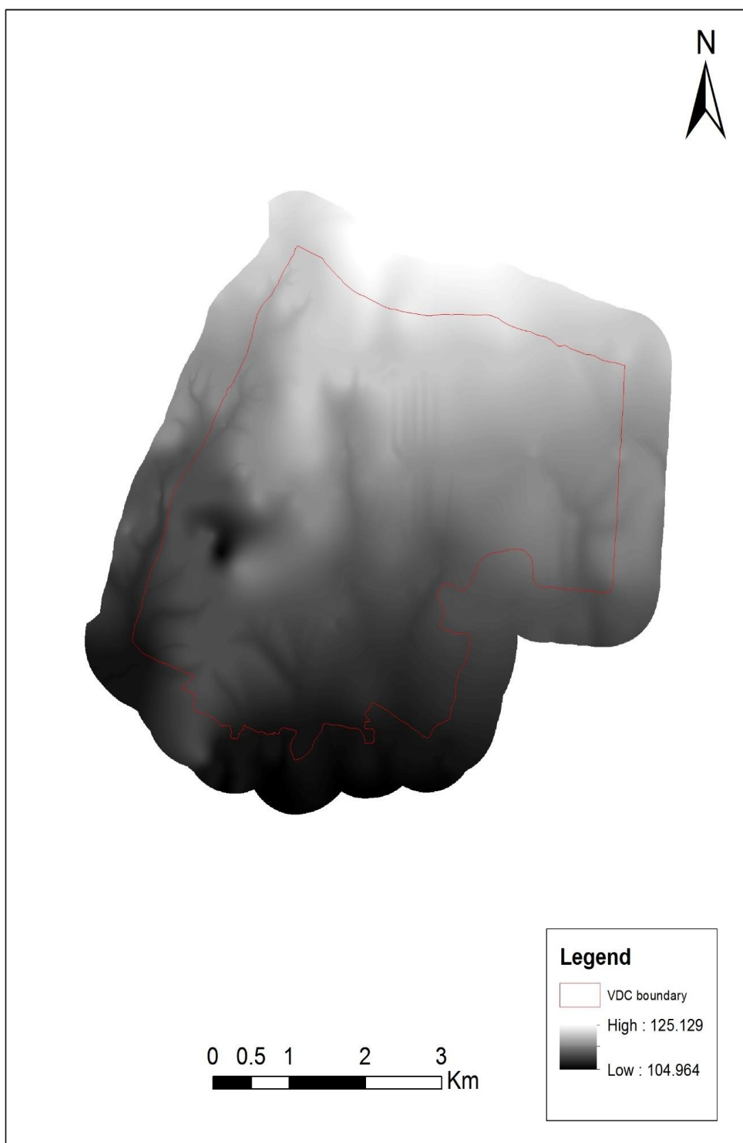
Figure 2.2: Digital elevation model of Anandaban VDC
