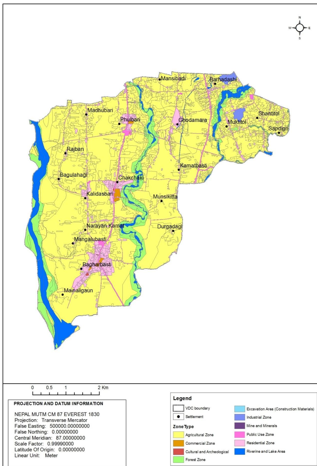
Figure 3.6 Land Use Zoning Map of Anandaban VDC
