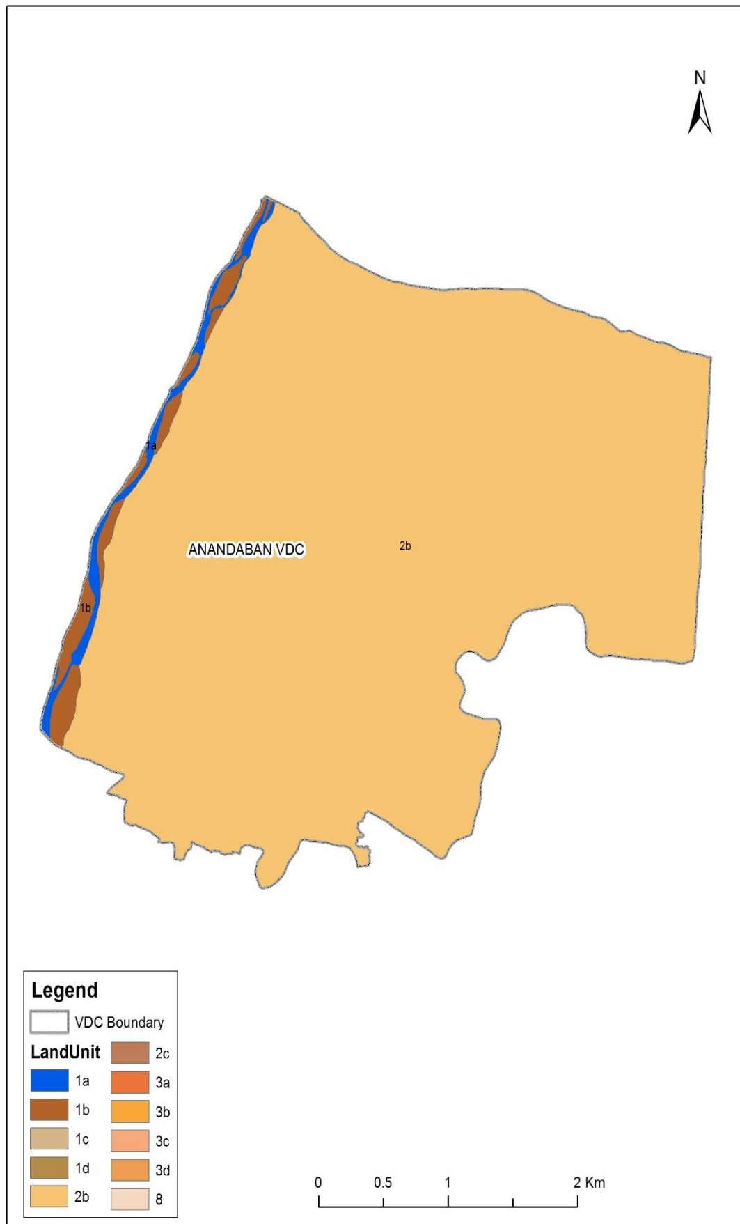
Figure 4.1: Land system map showing land units in Anandaban VDC
