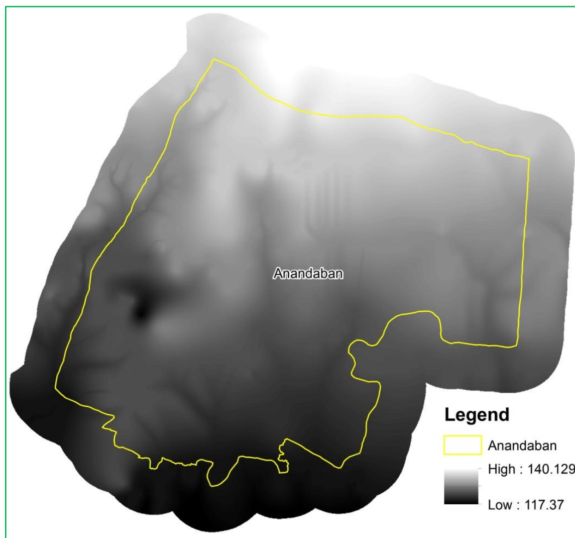
Figure 3.2 Anandaban VDC Boundary Overlaid on DEM
