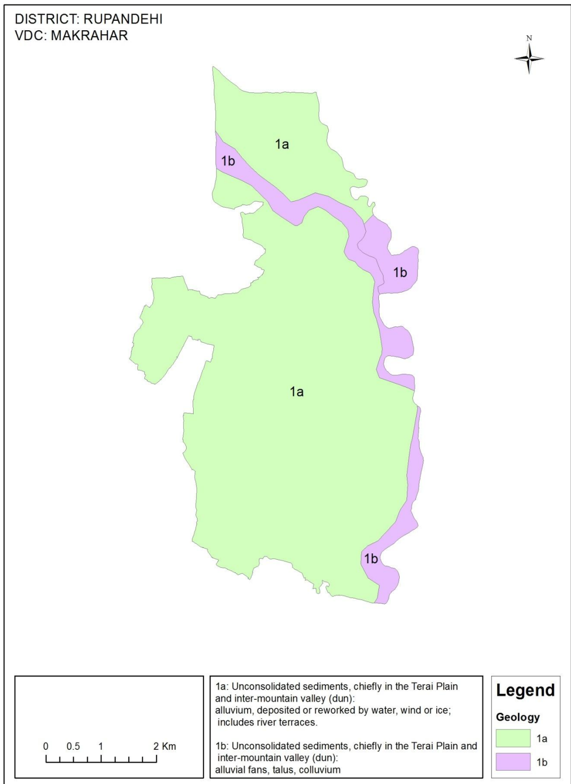
Figure 2.1: Geology Map of the MakraharVDC
