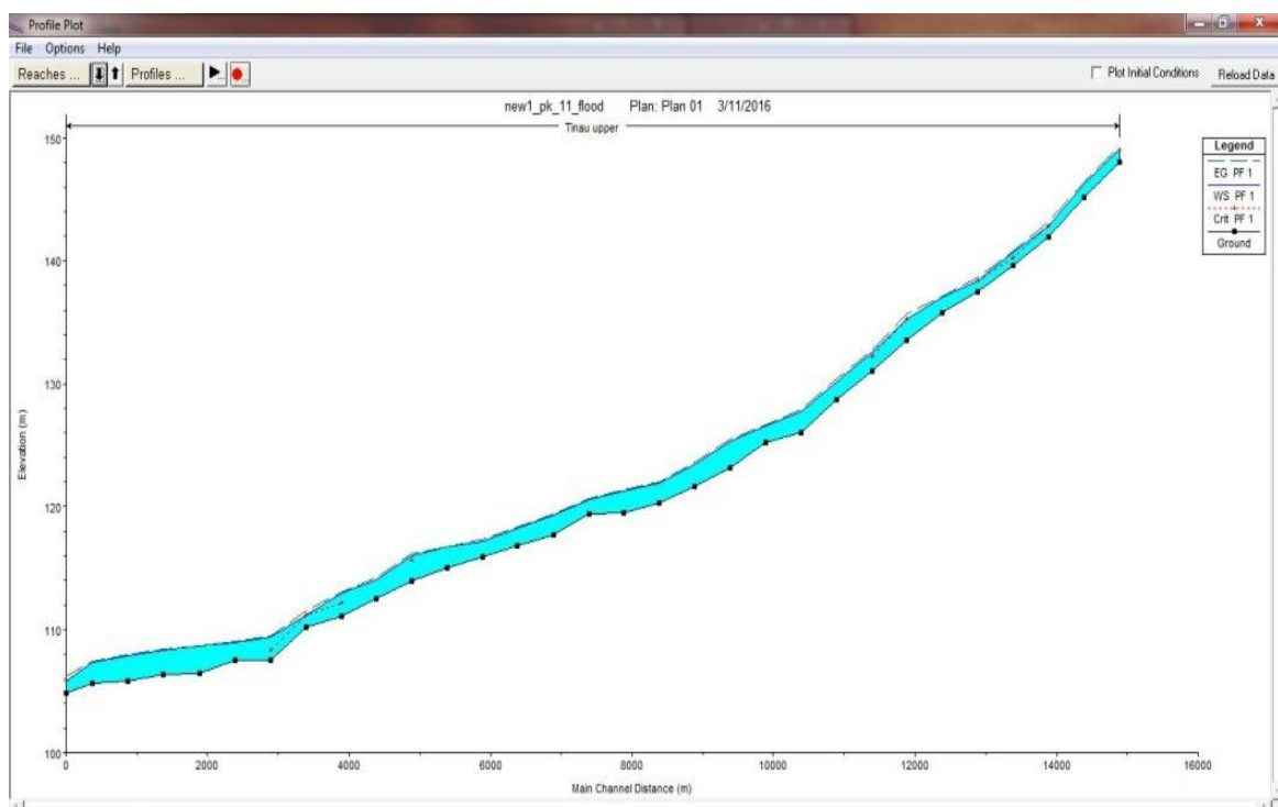
Figure 3.5 Water Surface Profile of TinauKhola for 100 Years
