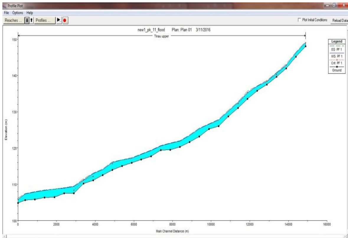
Figure 3.4 Water Surface Profile of TinauKhola for 100 Years
